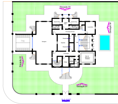
Subsolo A = 287,22 m 2
